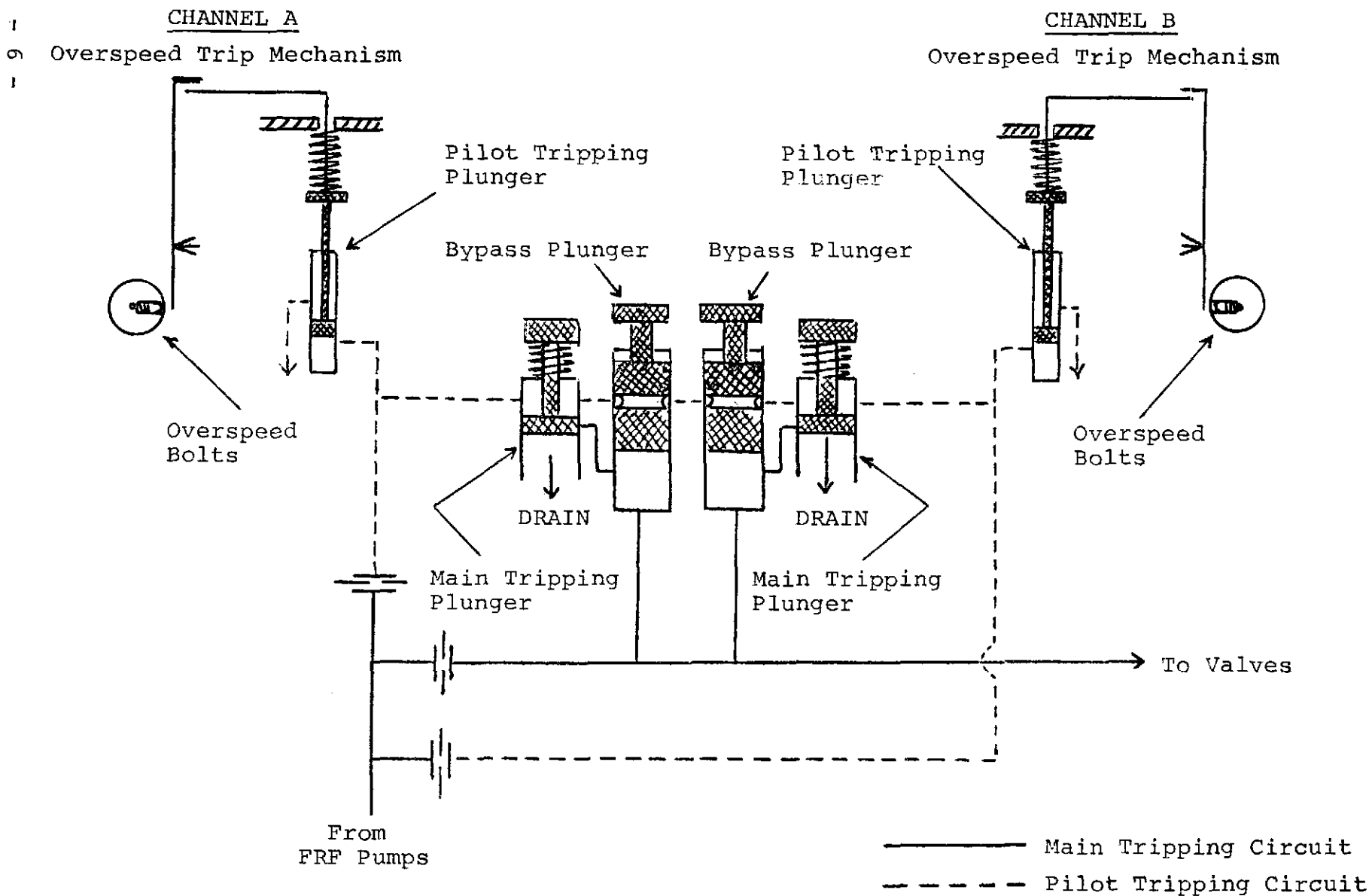
OVERSPEED TRIPPING CIRCUIT
