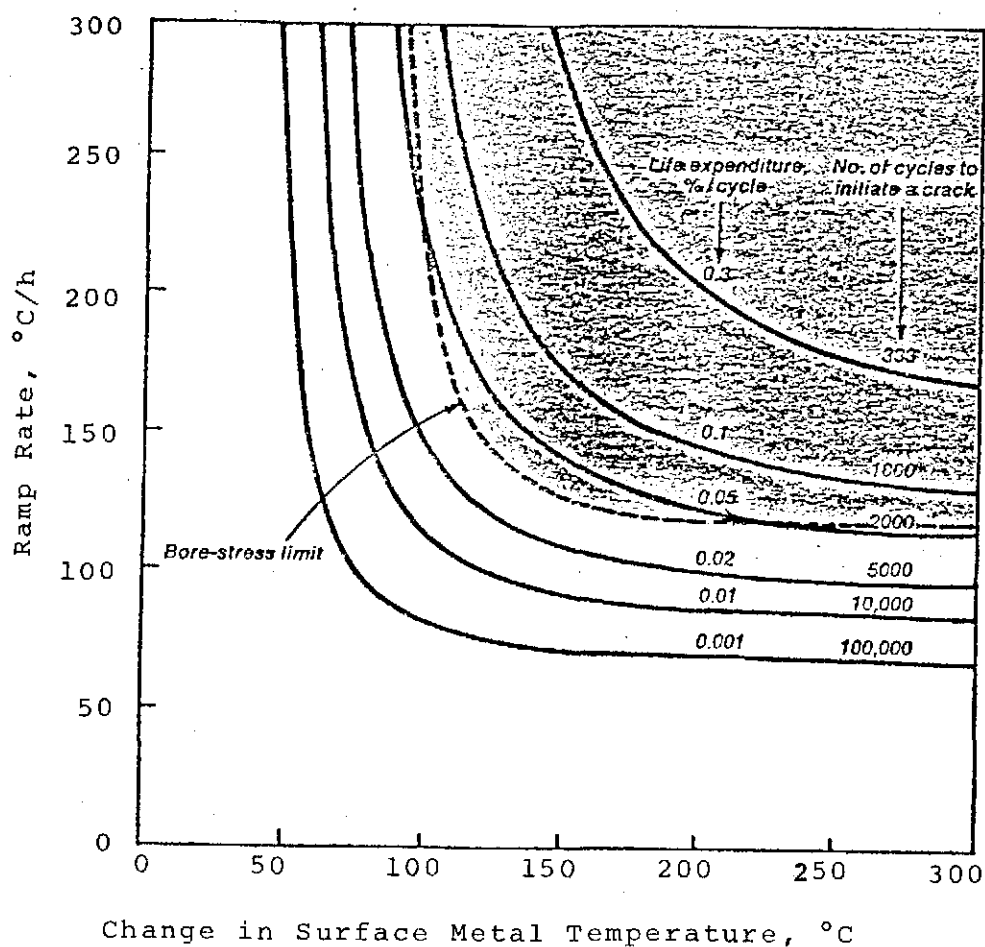
Cycle-Life Expenditure
