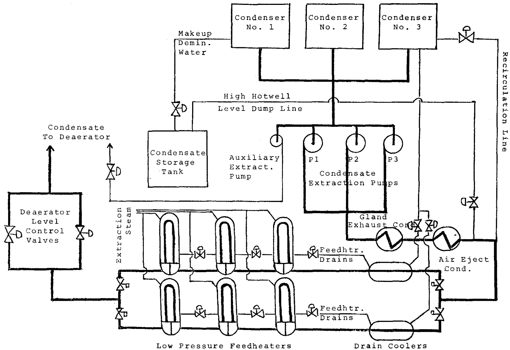
Figure 4.3 Condensate System
