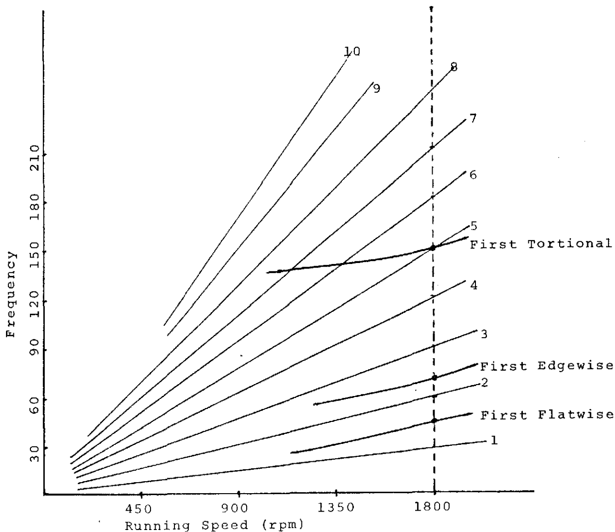
Campbell Diagram
